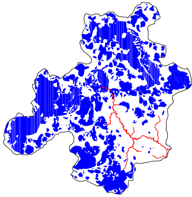
Figure 3.3.1-1A and 1B. Wetland Coverage in Seven Mile Creek in 1851 and 1985, respectively.
