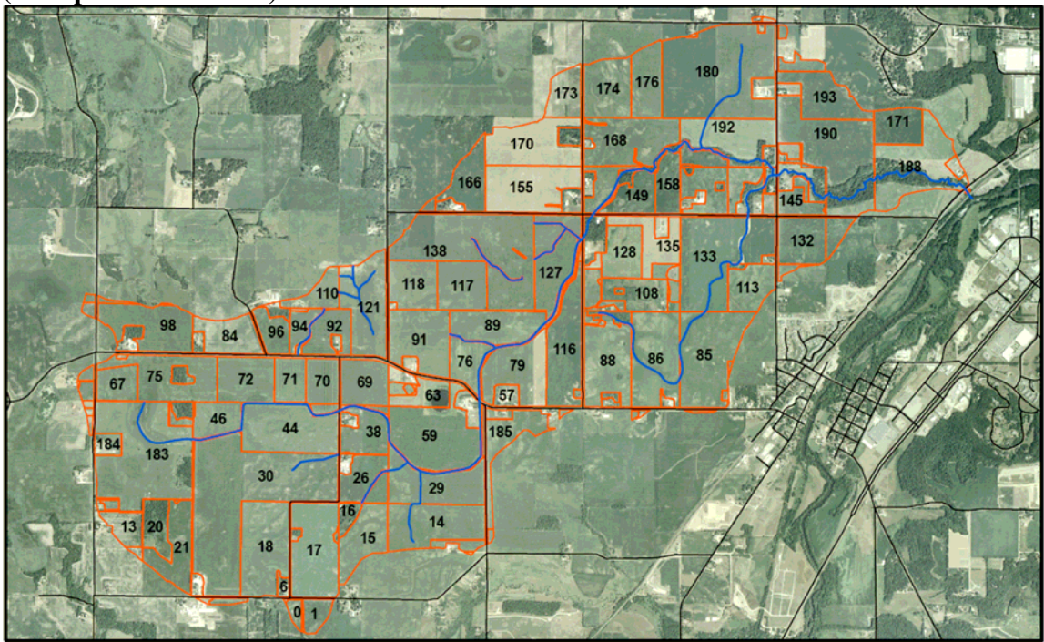
Figure 3.3.2-1. The Rice Creek Watershed Plotted Over a 2006 Aerial Photograph (with parcel numbers).
