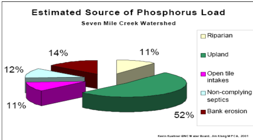
Figure 3.3.1-1 Estimated Sources of Phosphorus Load in Seven Mile Creek.
